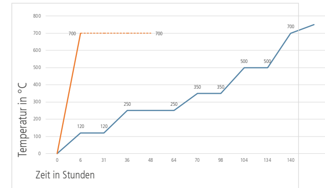
— Stampfmasse — INSURAL
