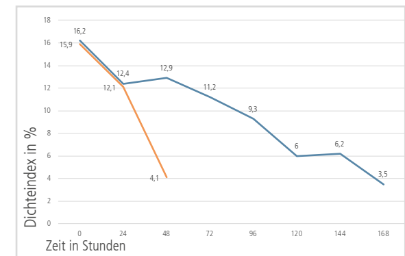
— Stampfmasse — INSURAL
