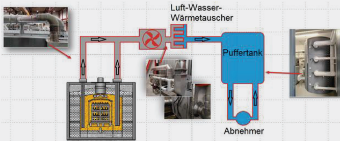
Fig. 1: Utilization of burner waste gases in a multi-purpose chamber furnace [2].
